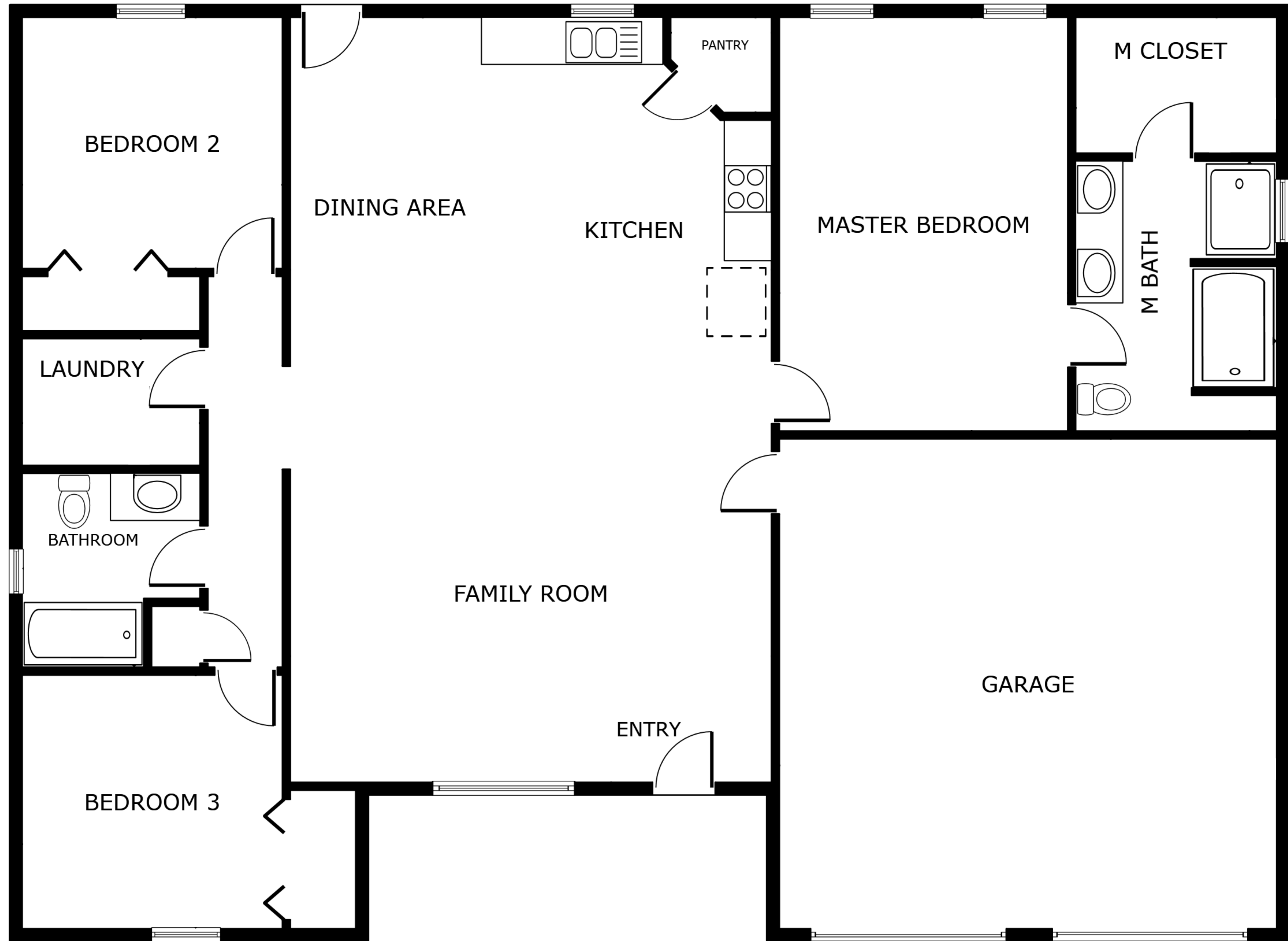
FLOOR PLAN
